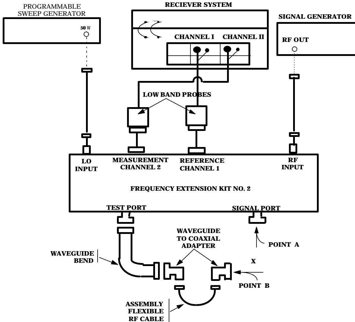
Figure 3. Equipment setup (26.5 to 40 GHz)
